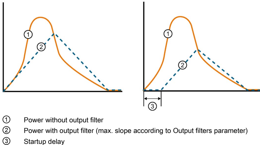
Figure 4-2 Power trend or average switch-on duration in case of phase control phase-angle proportional with and without output filter
