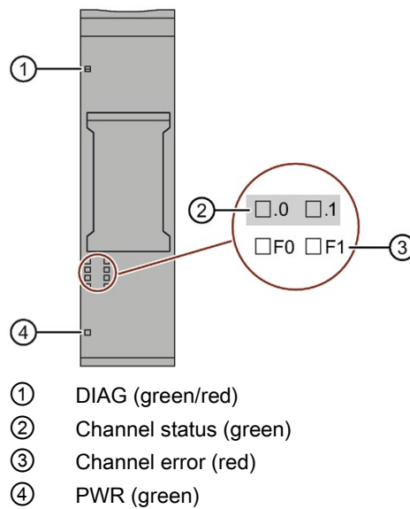
Figure 4-5 LED displays
