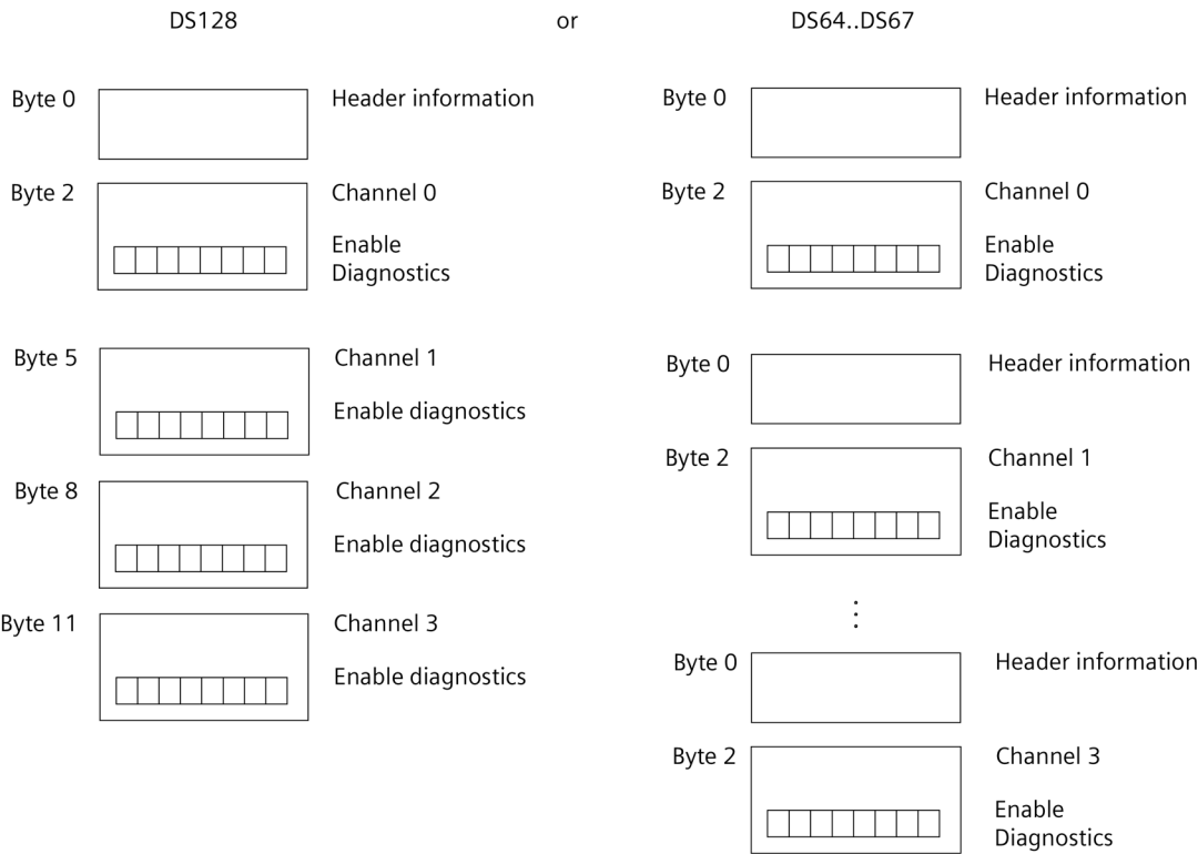
Figure A-1 Structure of data record 128 or data records 64 to 67
