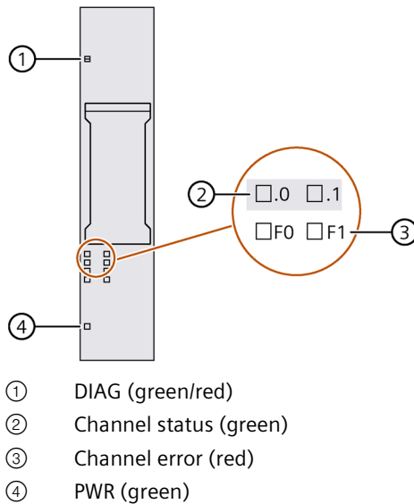
Figure 6-1 LED displays
