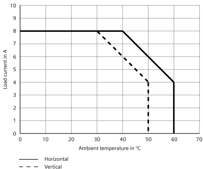
Figure 7-1 Load current vs. temperature in different mounting positions
