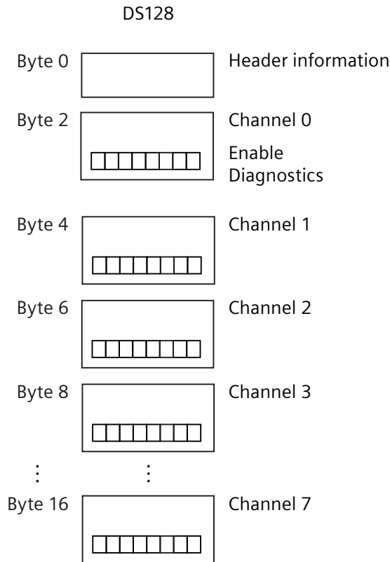
Figure A-1 Structure of data record 128
