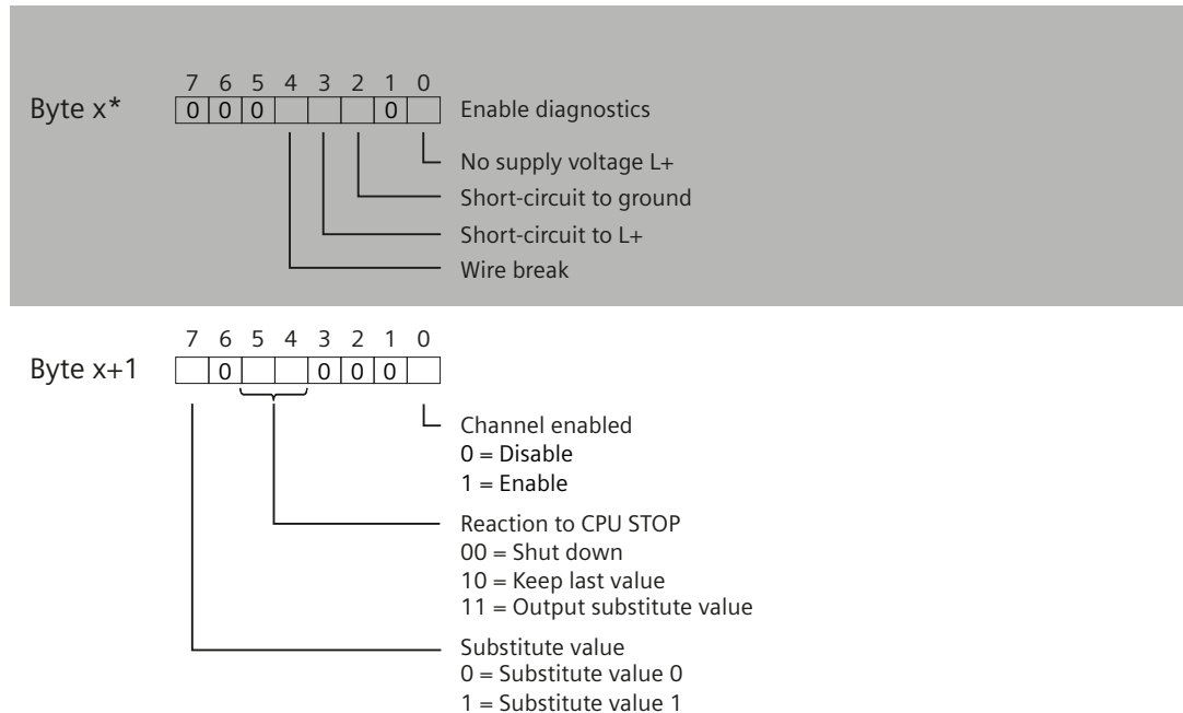
Figure A-3 Structure of byte x to x+1 for channels 0 to 7
