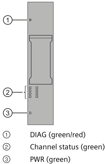
Figure 6-1 LED displays
