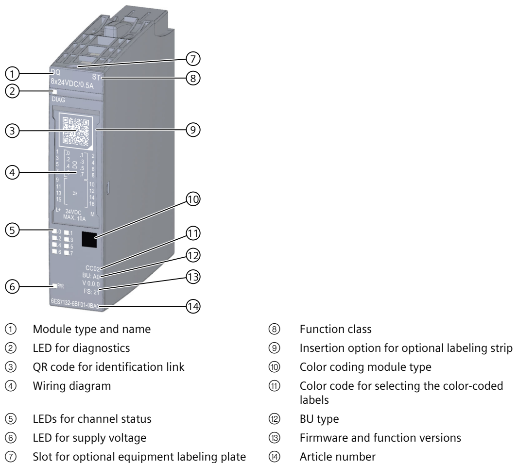
Figure 3-1 View of module DQ 8x24VDC/0.5A ST
