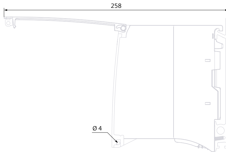
Figure A-2 CPU with open front panel
