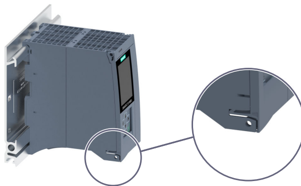
Figure 3-3 Locking latch on the CPU
