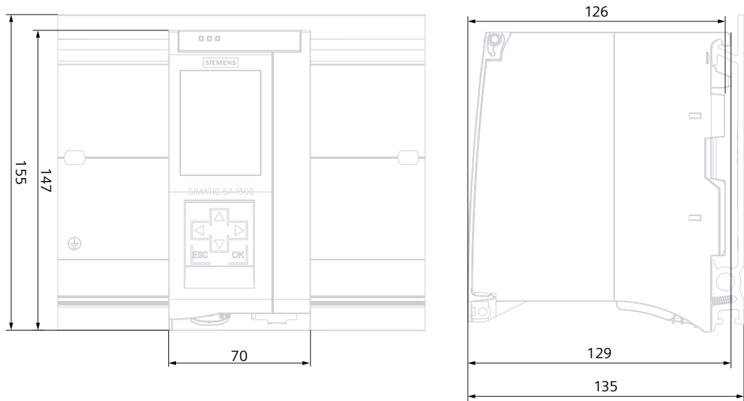
Figure A-1 Dimensional drawing of the CPU 1515-2 PN
