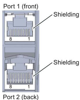
Figure 4-1 PROFINET
