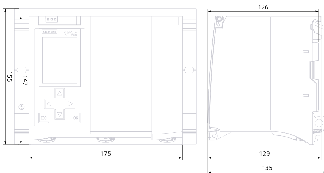
Figure A-1 Dimension drawing of the CPU 1517T-3 PN/DP, front and side view
