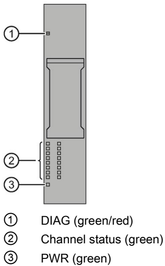
Figure 5-1 LED display
