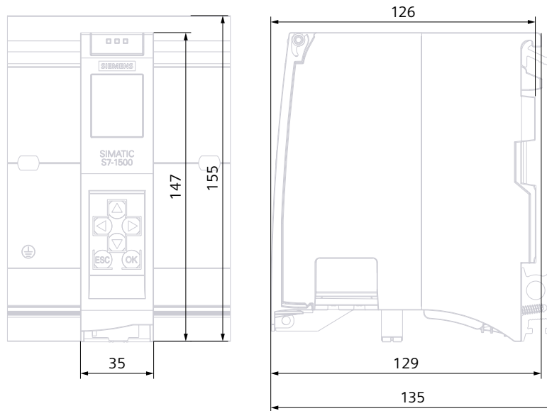
Figure A-1 Dimensional drawing of the CPU 1511T-1 PN, front and side view
