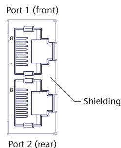
Figure 4-1 PROFINET ports
