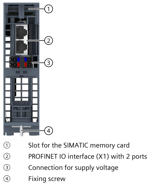
Figure 3-5 View of the CPU 1513-1 PN – bottom
