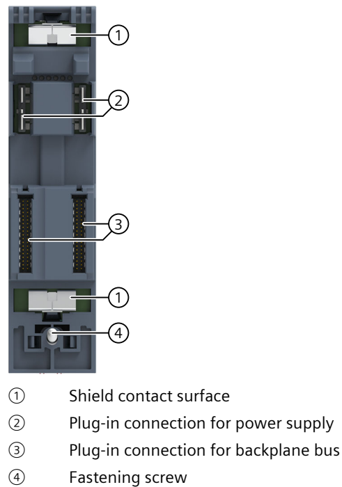
Figure 3-6 View of the CPU 1513-1 PN - rear
