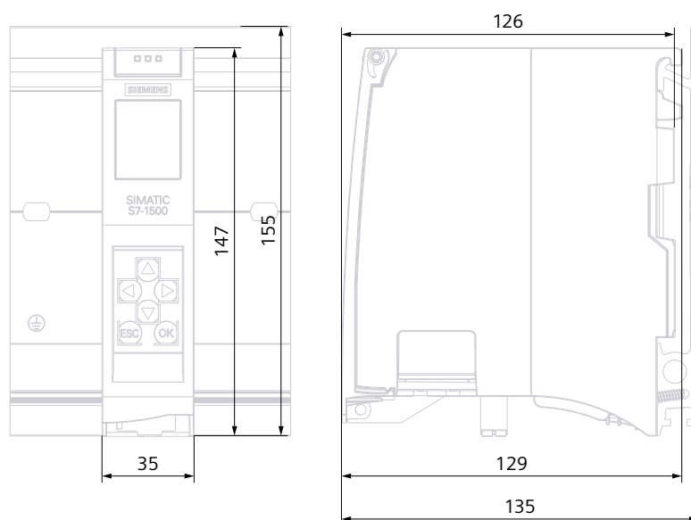
Figure A-1 Dimensional drawing of CPU 1513-1 PN, front and side views
