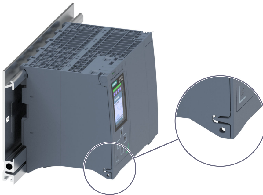
Figure 3-3 Locking latch on the CPU
