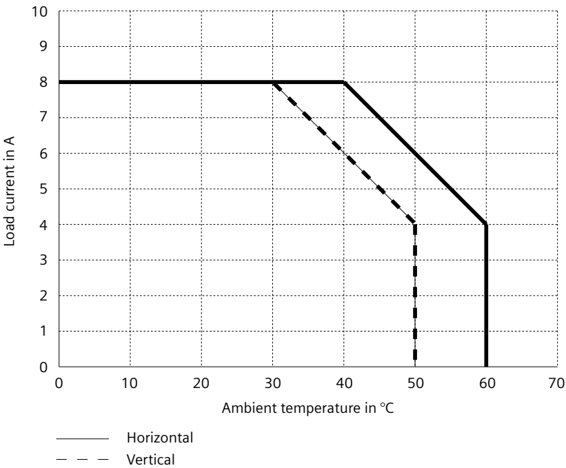
Figure 7-1 Load current to temperature in different installation positions
