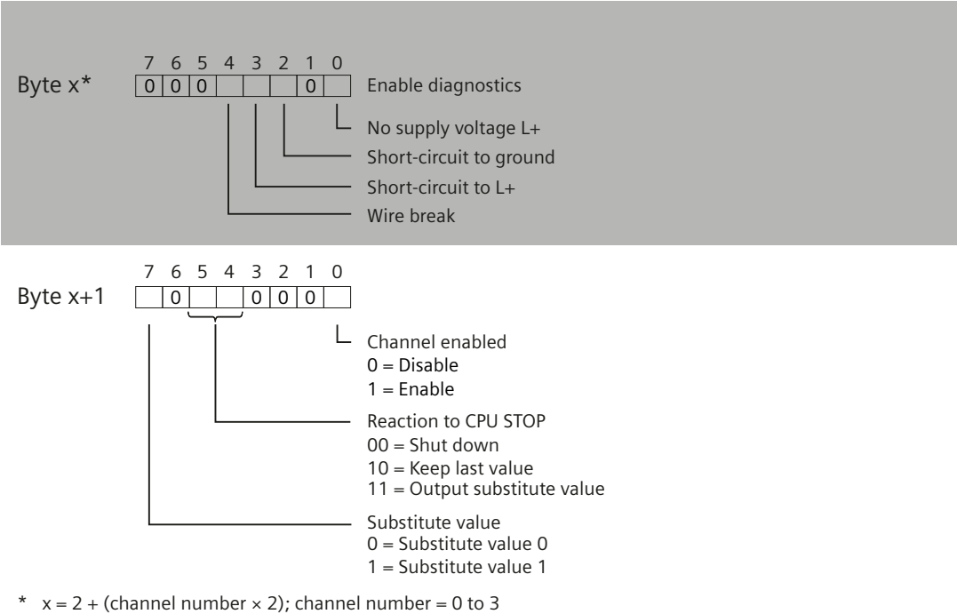
Figure A-3 Structure byte x to x+1 for the channels 0 to 3
